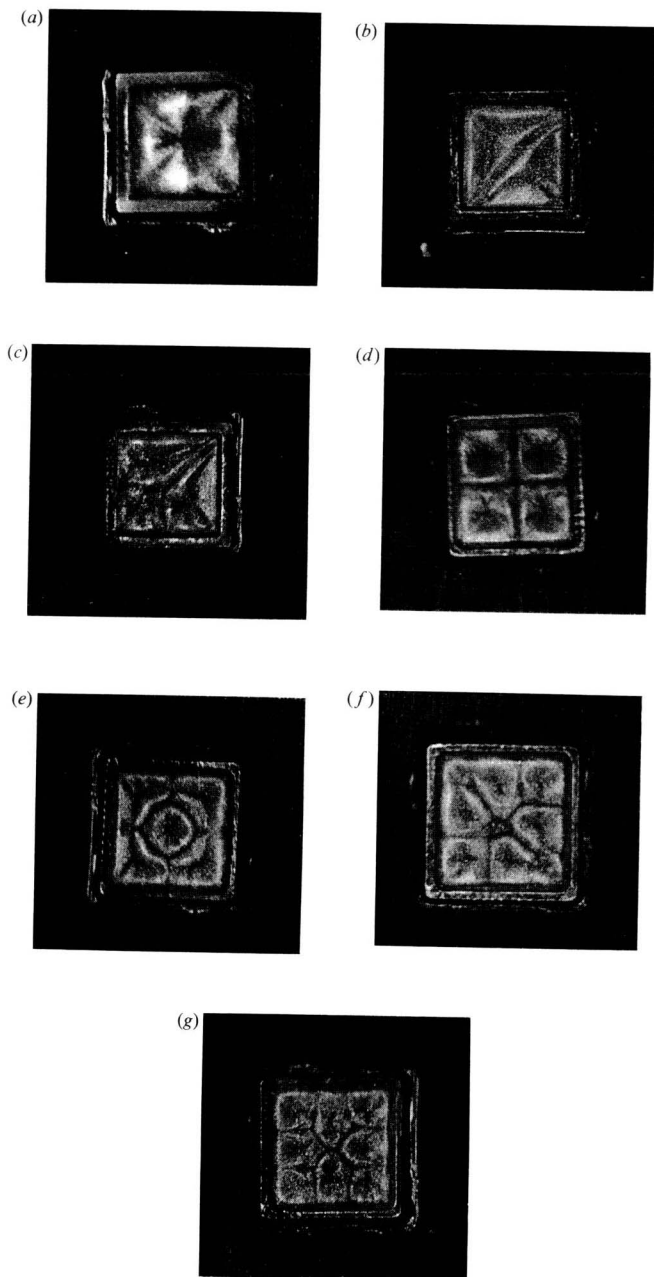
FIGURE 2. The patterns in the square container. (a) One-cell solution. Ma = 380 , R = 228 , A = 1.82 . (b) Two-cell solution. Ma = 54 , R = 33 , A = 5.68 . (c) Three-cell solution. Ma = 80 , R = 42 , A = 6.18 . (d) Four-cell solution. Ma = 78 , R = 38 , A = 6.36 . (e) Five-cell solution. Ma = 67 , R = 19 , A = 8.4 . (f) Six-cell solution. Just critical. Ma = 72 , R = 22 , A = 8.08 . (g) Eight-cell solution. Ma = 63 , R = 16 , A = 8.75 .
