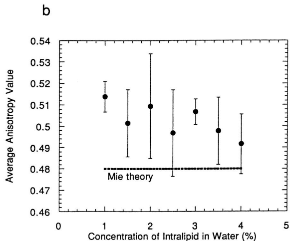
Fig. 3 The anisotropy at 1064 nm for varying concentrations of water suspensions of (a) India ink and (b) Intralipid-10%. The Mie theory value is taken from Ref. 5.
