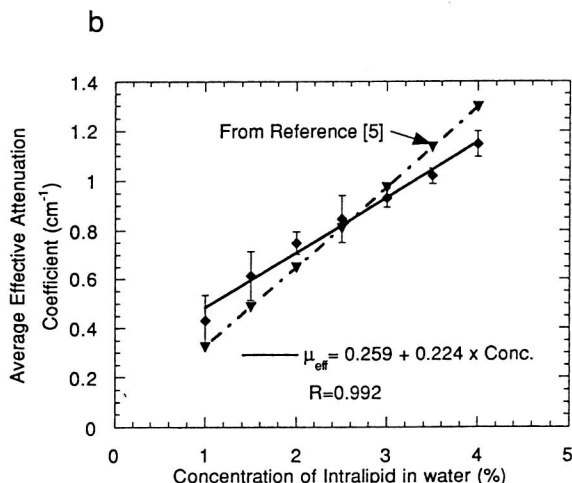
Fig. 4 The attenuation coefficients at 1064 nm for varying concentrations of water suspensions of (a) India ink and (b) Intralipid-10%. The total attenuation coefficient is plotted for the India ink's highly absorbing suspensions. The effective attenuation coefficient is plotted for Intralipid's highly scattering suspensions. The dotted plot in (b) is taken from data in Ref. 5.
