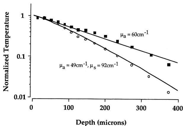
Fig. 6 The calculated internal temperature distribution for absorbing-only and turbid samples. The solid curves represent analytical solutions for the internal temperature given by Beer's law for an absorbing-only and by diffusion theory for a turbid sample. The predicted temperatures are accurate up to one-tenth of the maximum temperature. The temperatures are normalized to the maximum surface temperature detected.
