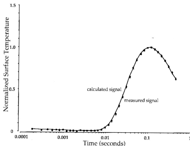
Fig. 11 Identical normalized surface signals from the measured and calculated profiles in Figure 7(b). This figure illustrates multiple solutions to the matrix equation (8).
