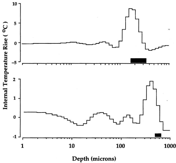
Fig. 8 The calculated internal temperature distribution for a 170 \mu\text{m} gel layer buried at 170 \mu\text{m} and 510 \mu\text{m} under clear gel layers. The layer is represented by the black bar below the temperature profiles. The absorption of the layer is 400\text{ cm}^{-1} . The algorithm works well for identifying the depth of the impulses, but does not do very well at predicting the magnitude of the temperature.
